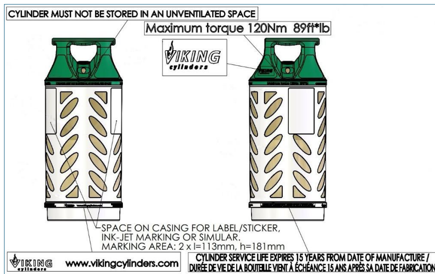
Figure 4-1 - Example casing markings
